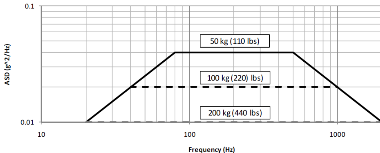
Figure 2—Mass Attenuated Workmanship Vibration Spectrum
