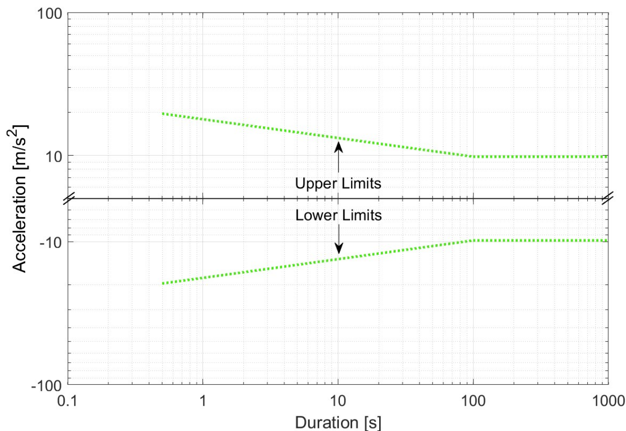
Figure 6.5-6—Ay Sustained Translational Acceleration Limits (Standing)
