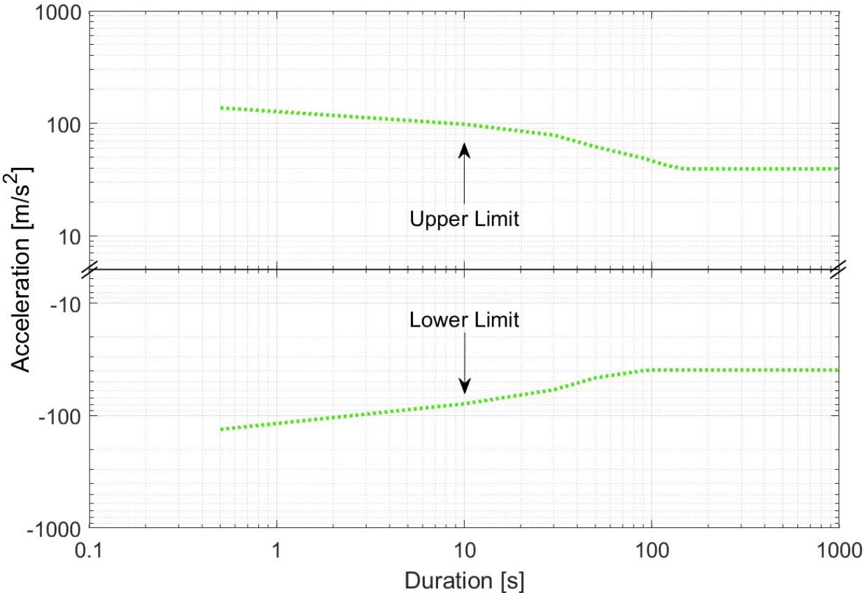
Figure 6.5-5—Ax Sustained Translational Acceleration Limits (Standing)
