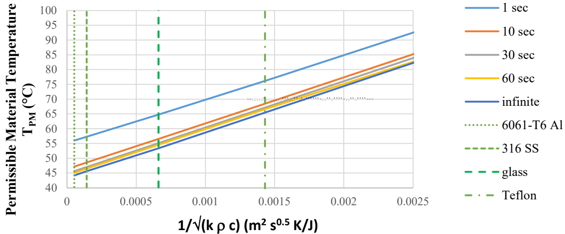
Figure 9.3-3—High T_{PM} for Incidental and Intentional (Planned) Contact (43°C)
