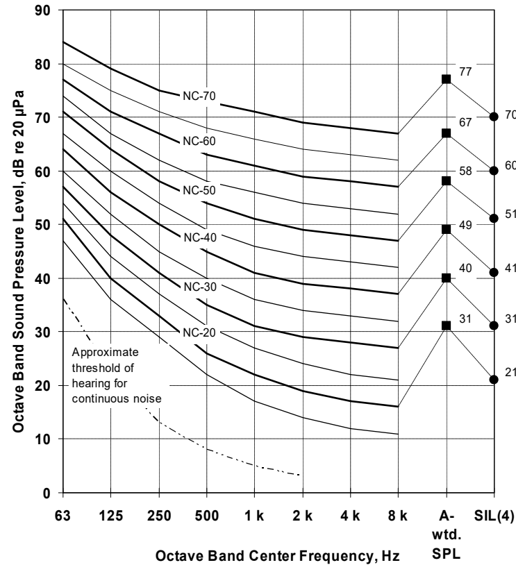
Figure 6.6-1—NC Curves
