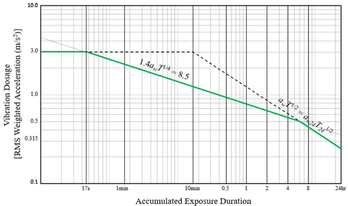
Figure 6.7-2—Long-Duration Vibration Dosage Limits for Health during Non-Sleep Phases of Mission
