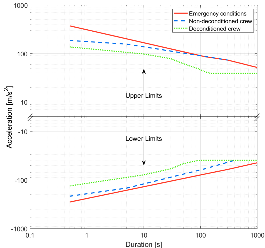
Figure 6.5-2—Ax Sustained Translational Acceleration Limits (Seated)
