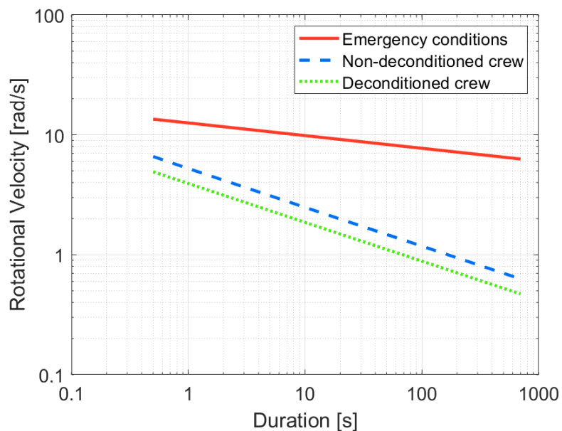
Figure 6.5-8—Rotational Velocity Limits
