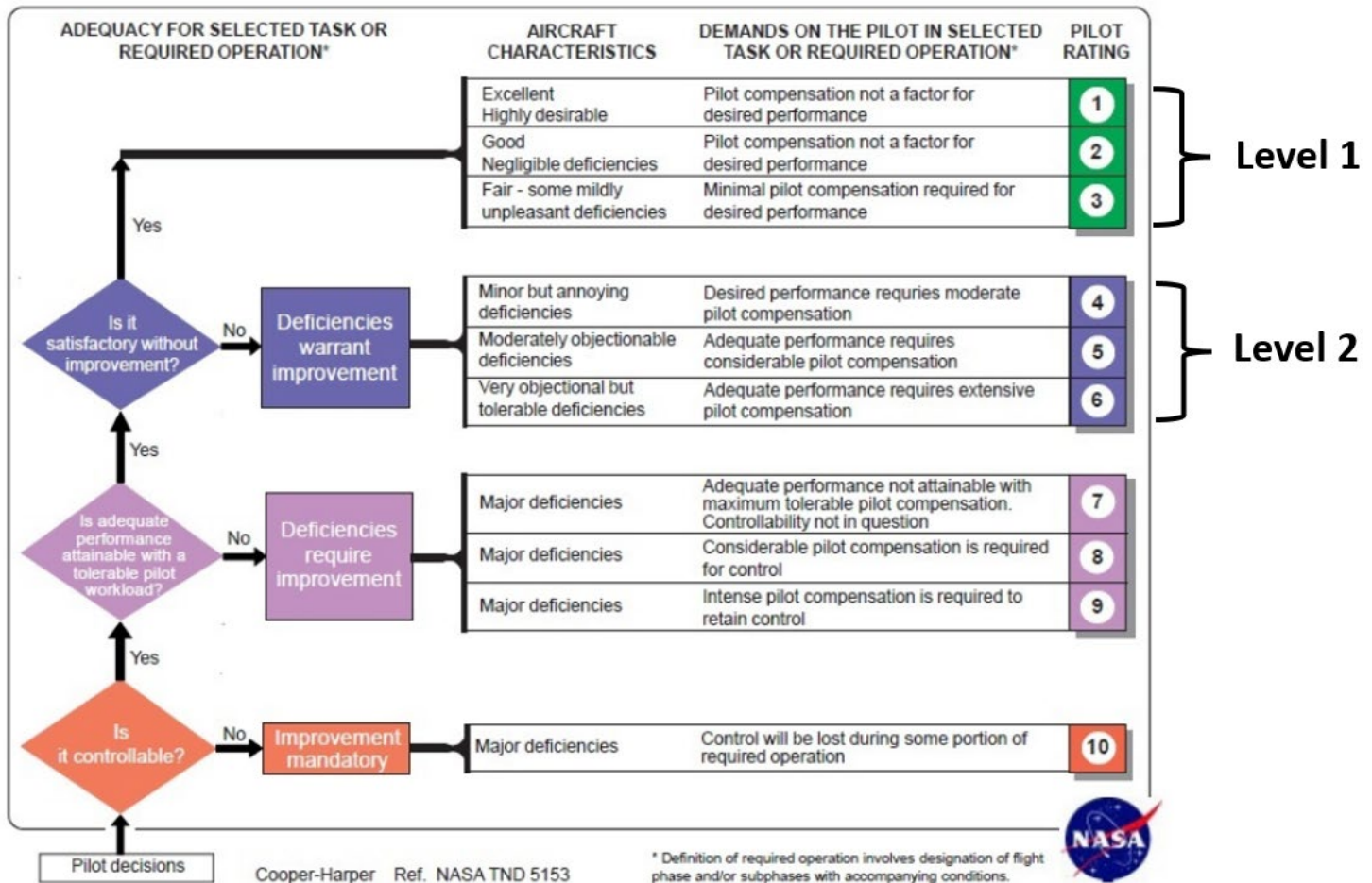
Figure 5.1-2—Cooper-Harper Handling Qualities Rating Scale
