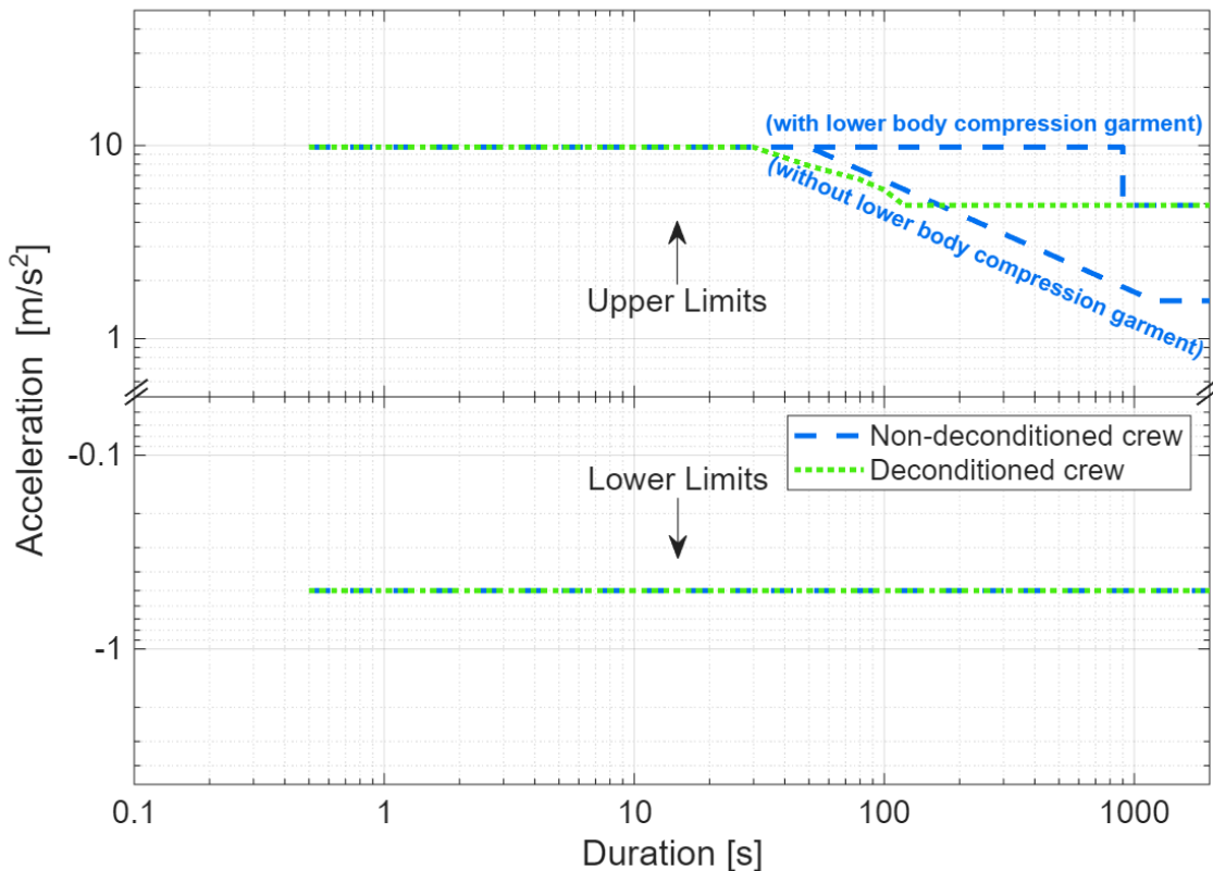
Figure 6.5-7—Az Sustained Translational Acceleration Limits (Standing)
