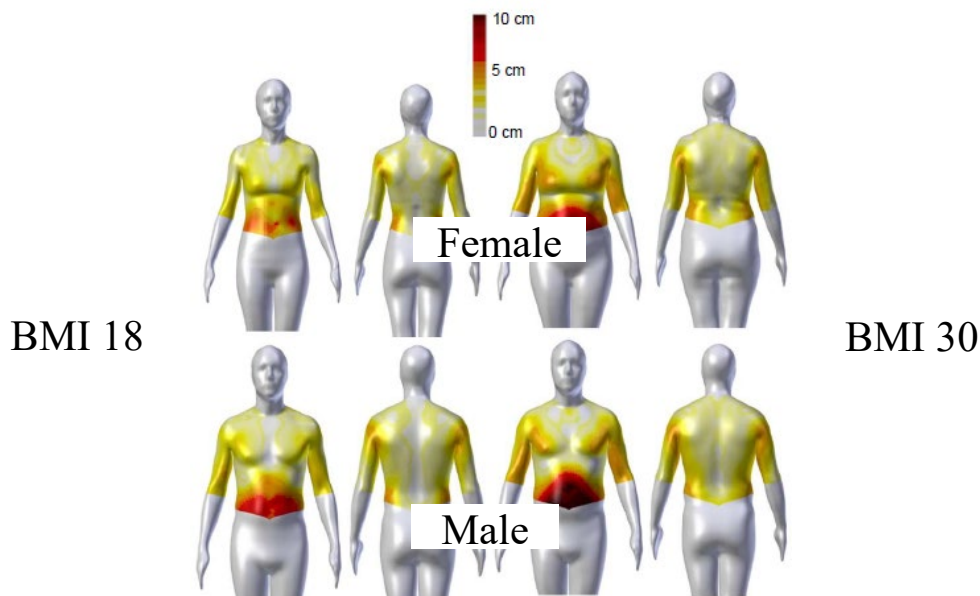
Figure 6.5-9—Performance Blunt Force Maximum Allowable Depth of Compression Limits (Seated or Standing Vehicle Occupants)
