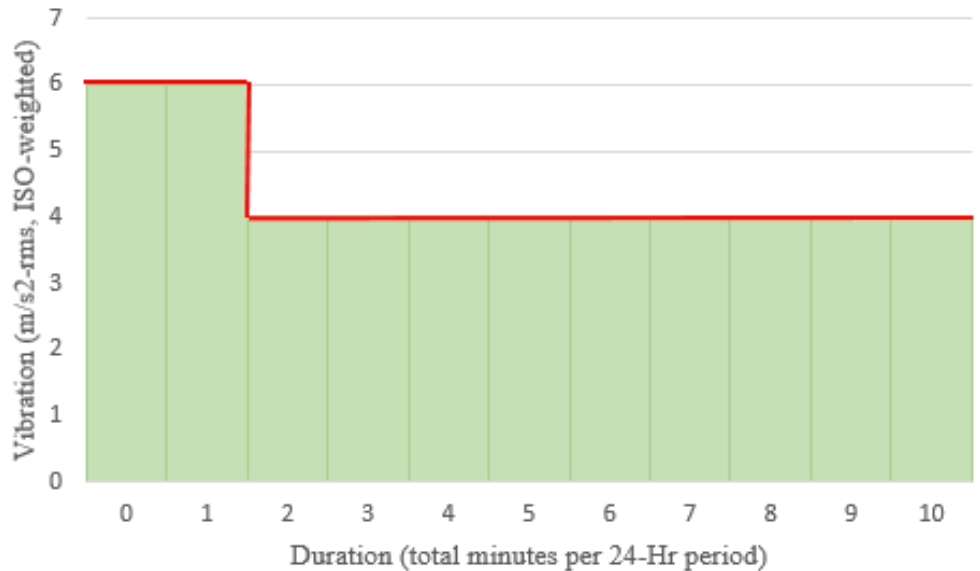
Figure 6.7-1—Frequency-Weighted Vibration Limits by Exposure Time during Dynamic Phases of Flight
