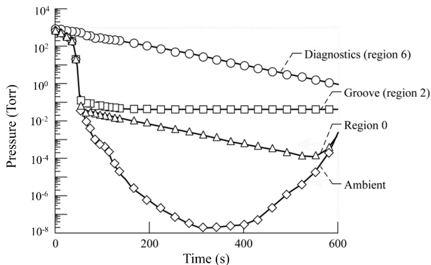
Figure 5—Payload Pressure for a Vented Payload During Launch
