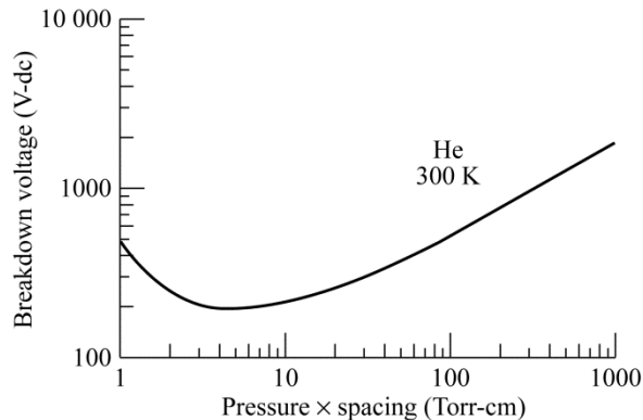
Figure 13—Paschen Curve of Helium as a Function of pd at Room Temperature
