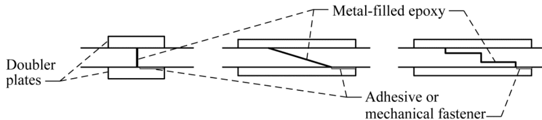
Figure 78—Butt, Scarf, and Stepped Lap Joints
