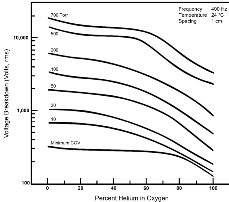
Figure 23—Parallel Plates in Helium-Oxygen
