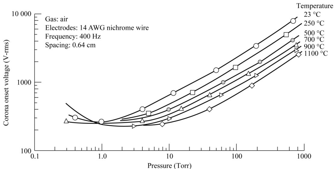
Figure 16—Corona Between Nichrome Wires in Heated Chamber
