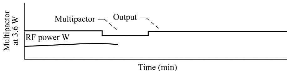
Figure 31—Power Decrease Caused by Multipactor
