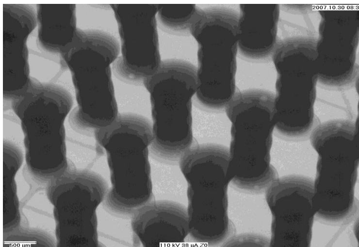
Figure 1- Example of an Oblique X-ray view showing an Acceptable level of voiding in the solder joints.
