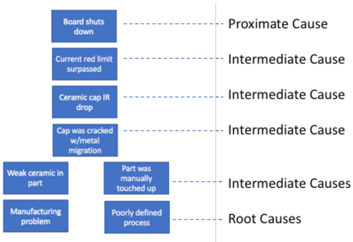
Figure 1. Fault tree representing logic flow for example
