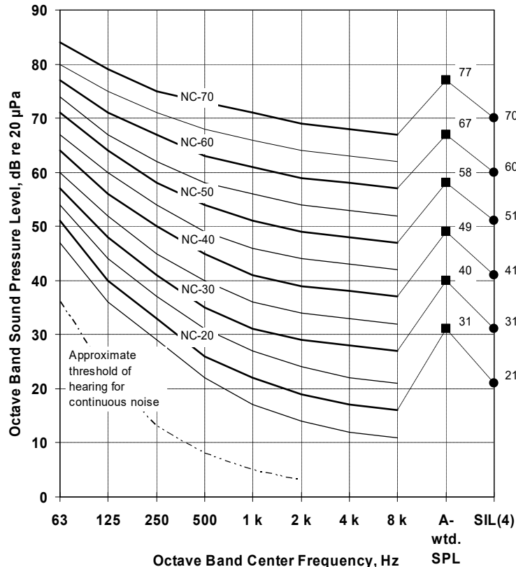
Figure 6.6-1—NC Curves
