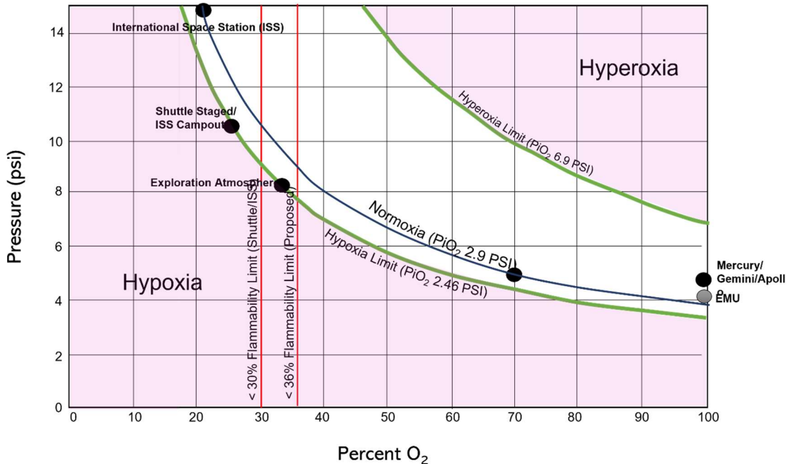
Figure 6.2-1—Atmospheric Composition
