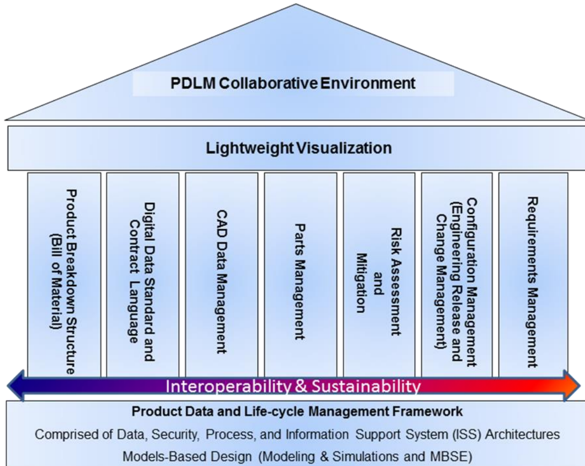
Figure 2—PDLM Framework
