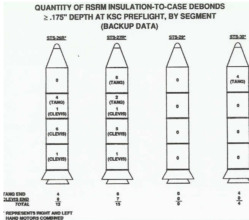
Figure E.5-10: Quantity of RSRM Insulation-to-Case Debonds ≥ 0.175" Depth at KSC Preflight, by Segment (Backup Data)
