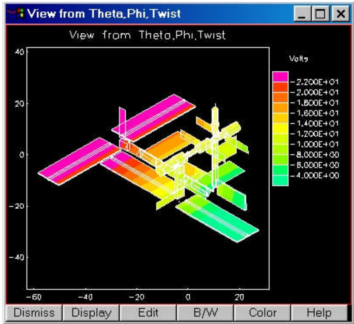
Figure 12— An EWB Contour Plot of ISS Potentials (This is the 12A mission configuration at an arbitrary point in the orbit. The deviation from right-front to left-rear in the picture is due to \vec{v} \times \vec{B} \cdot \vec{l} effects. In this picture, the velocity is toward the lower left, and the magnetic field is somewhat vertical. Taken from Ferguson and Hillard, 2003.)
