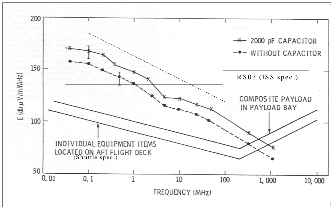
Figure 10—EMI from a Small Solar Array Arc and a Hypothetical ISS Anodized Aluminum Arc Compared to Orbiter’s Specs (after Leung, 1985)
