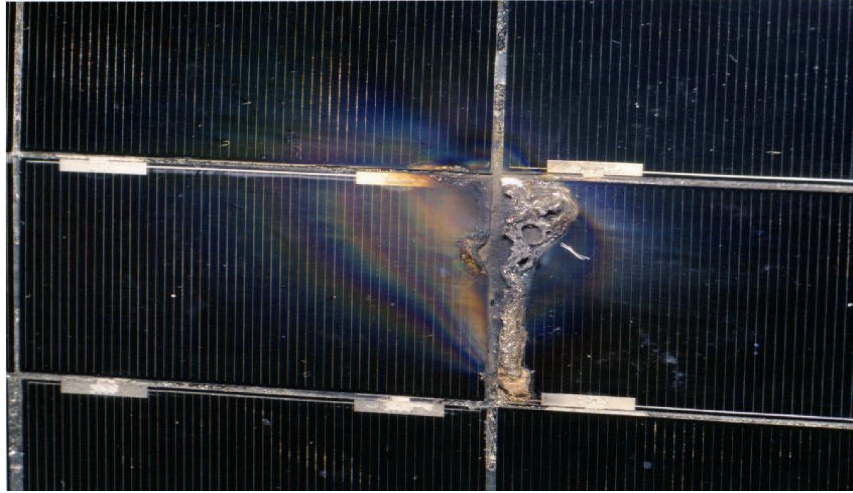
Figure 7—Arc Site of Sustained Arc on EOS-AM1 Sample Array. Cells are 2x4 cm. (Ferguson and Hillard, 2003)
