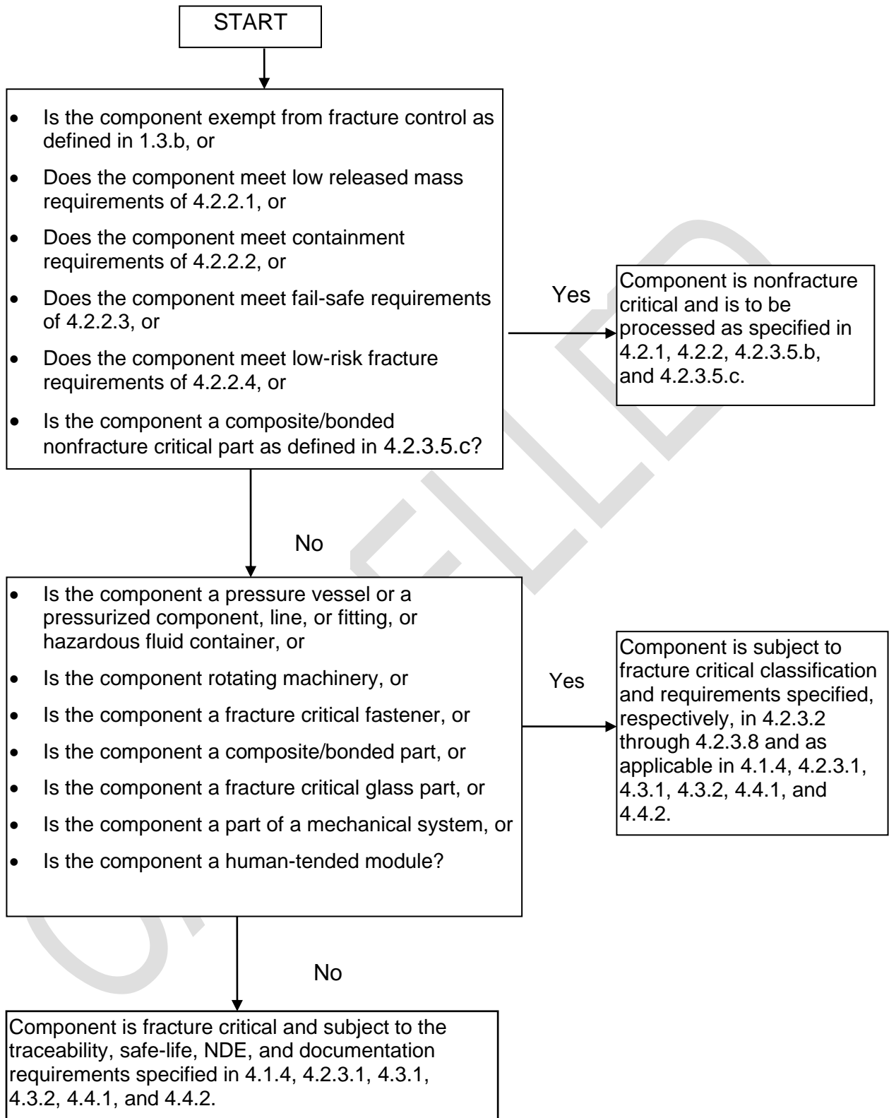
FIGURE 1. Fracture Control Classification/Processing of Payload Components
