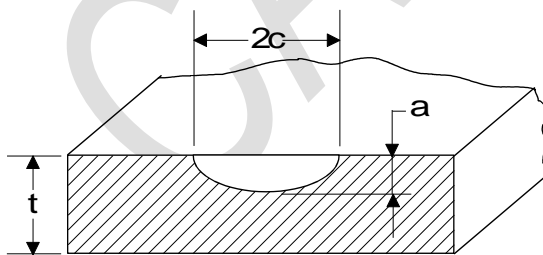
SURFACE CRACK
