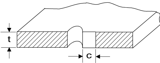
THROUGH CRACK
