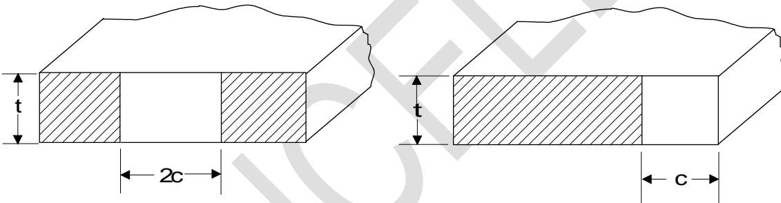
THROUGH CRACKS
