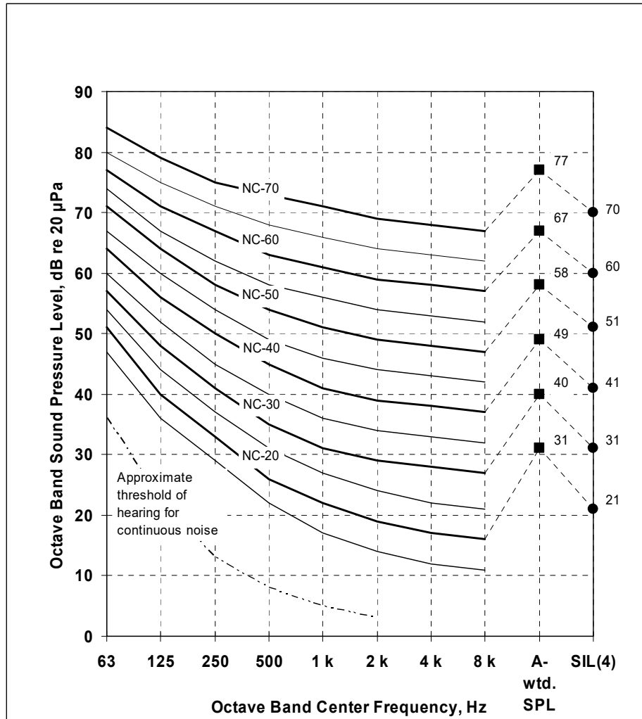
Figure 9—NC Curves
