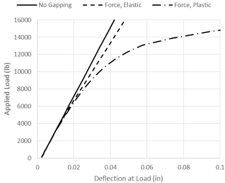
Figure 26—System Stiffness Due to Separation and Yielding
