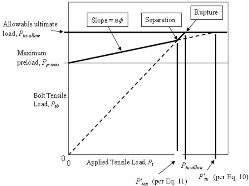
Figure 14—Separation before Rupture with Linear Theory
