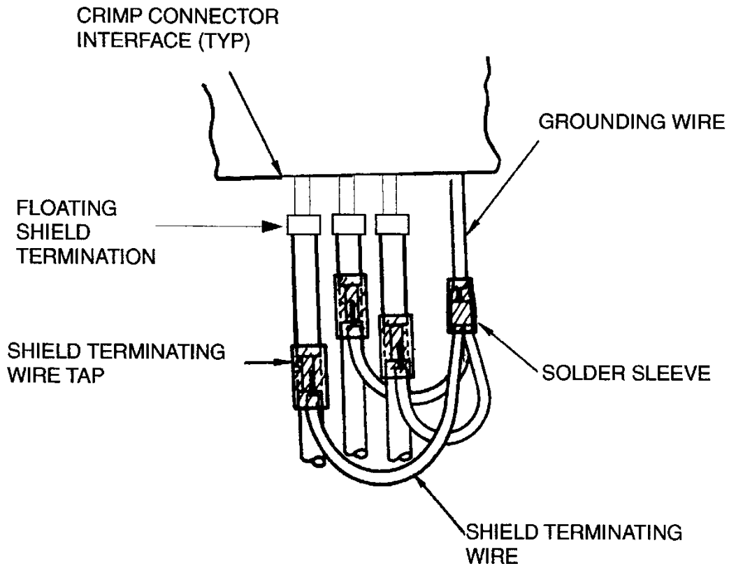
Figure Error! No text of specified style in document.-21. Example of Group Grounding of Staggered Shields
