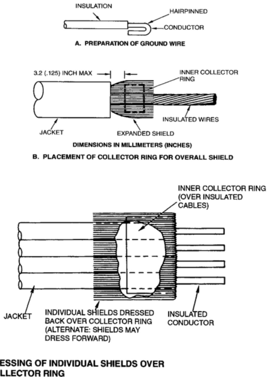
Figure Error! No text of specified style in document.-23. Large Compression Ring Grounding (Typical Applications)
