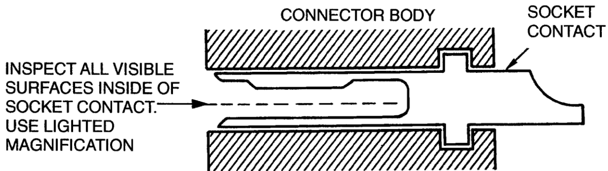
Figure Error! No text of specified style in document. -29. Visual Examination Inside the Socket Contact for Flux Residue
