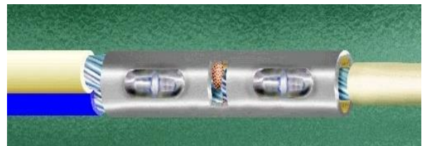
Figure Error! No text of specified style in document.-59. Properly Crimped Butt Splice
