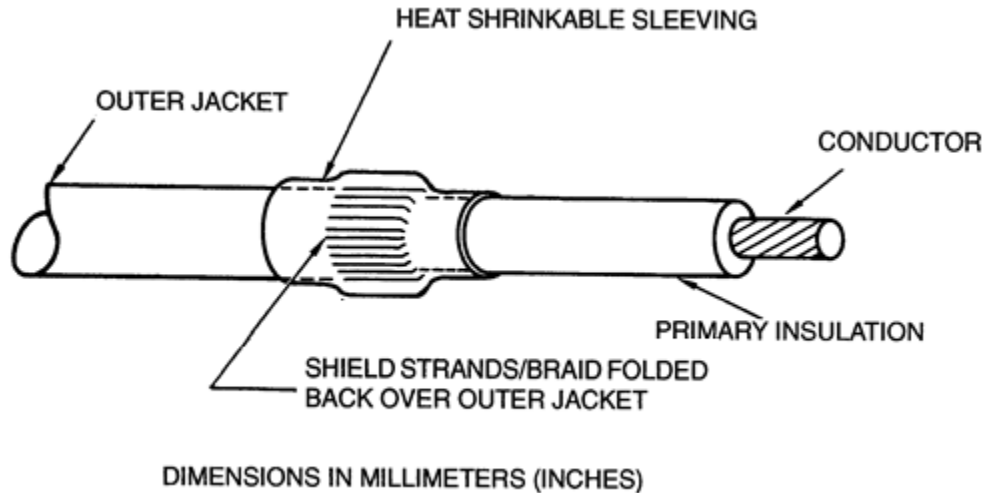
Figure Error! No text of specified style in document. -24. Floating Shield Termination
