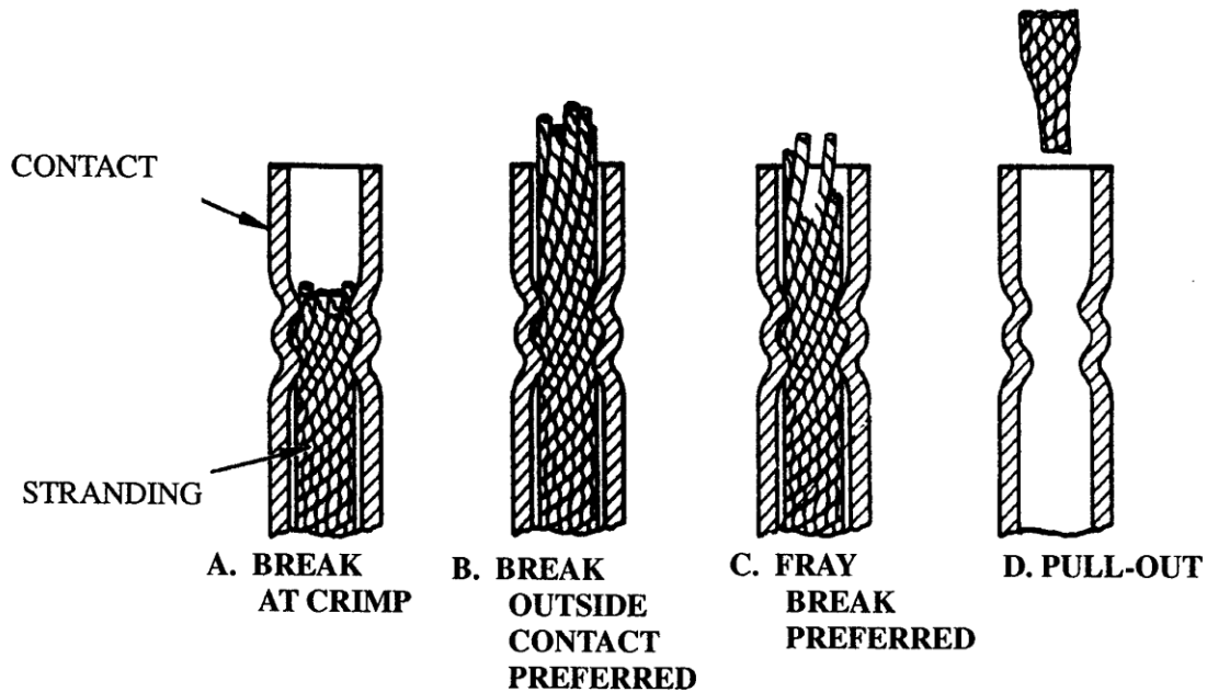
Figure Error! No text of specified style in document.-26. Crimp Joint Tensile Failure Categories
