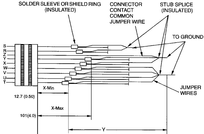
Figure Error! No text of specified style in document.-22. Group-Grounding of Individual Shield Terminations
