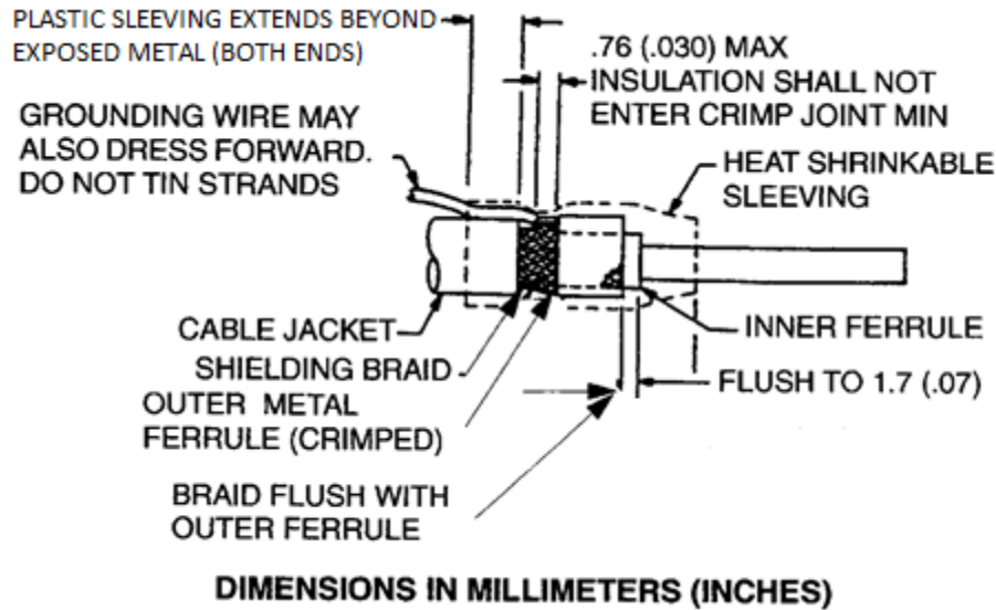
Figure Error! No text of specified style in document.-20. Individual Shield Termination Using a Two-Piece Crimp Ring
