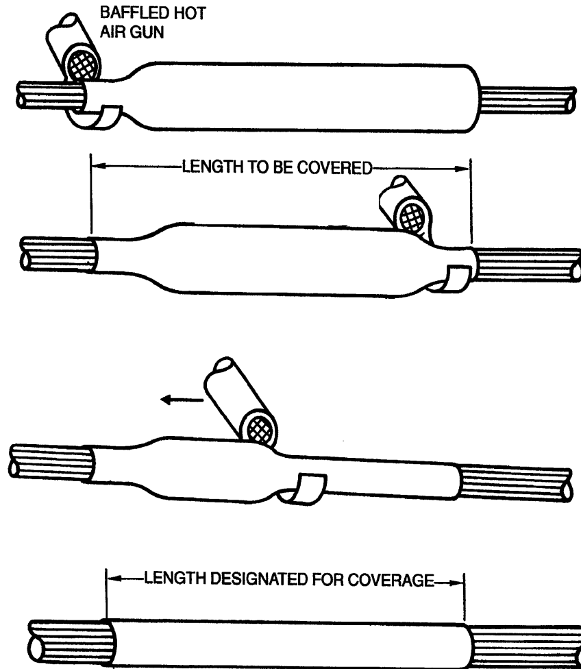
Figure Error! No text of specified style in document. -16. Installation of Long Lengths of Sleeving to Achieve Controlled Dimensions
