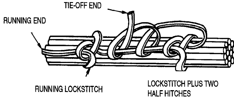
Figure Error! No text of specified style in document.-5. Closing Stitch and Single Tape— Illustration
