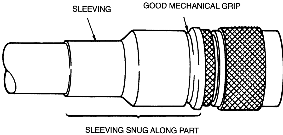
Figure Error! No text of specified style in document.-17. Sleeving Installation (Typical)
