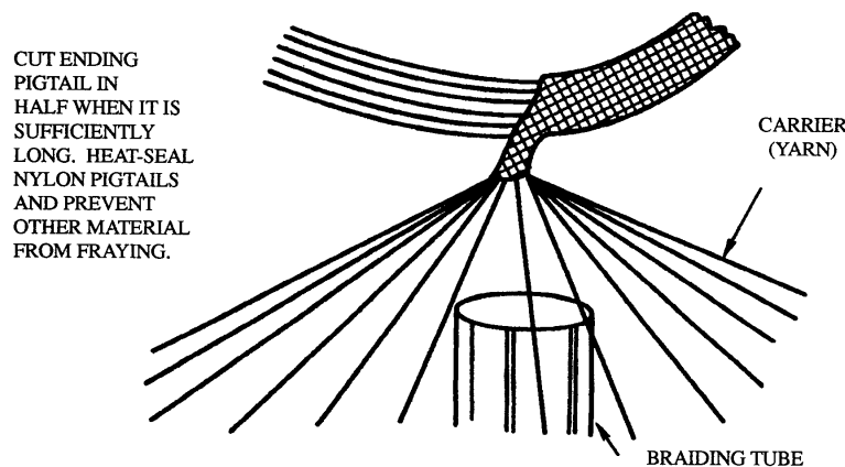
Figure Error! No text of specified style in document.-11. Forming Ending Pigtail
