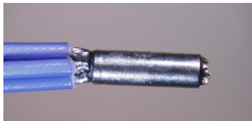
Figure Error! No text of specified style in document.-49. Solder Ferrule
