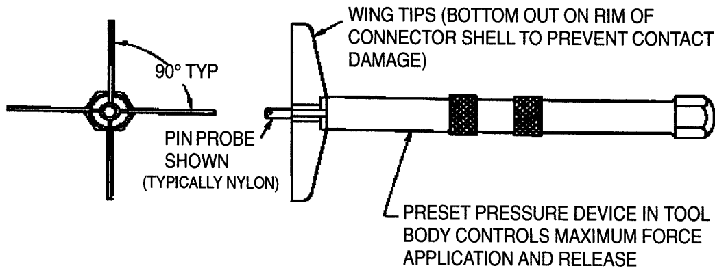
Figure Error! No text of specified style in document.-27. Typical Push Test Tool
