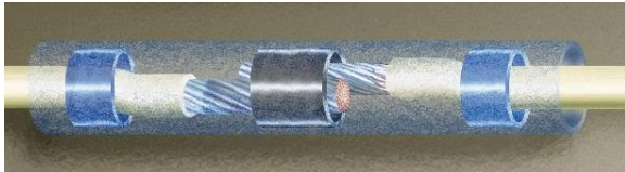
Figure Error! No text of specified style in document. -42. Solder Sleeve Prior to Flow
