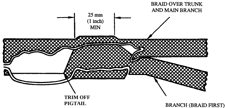
Figure Error! No text of specified style in document.-12. Braiding at a Breakout or Y Intersection
