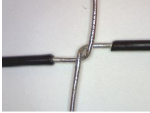
Figure Error! No text of specified style in document. -45. Initial Wrap for Western Union/Lineman Splice
