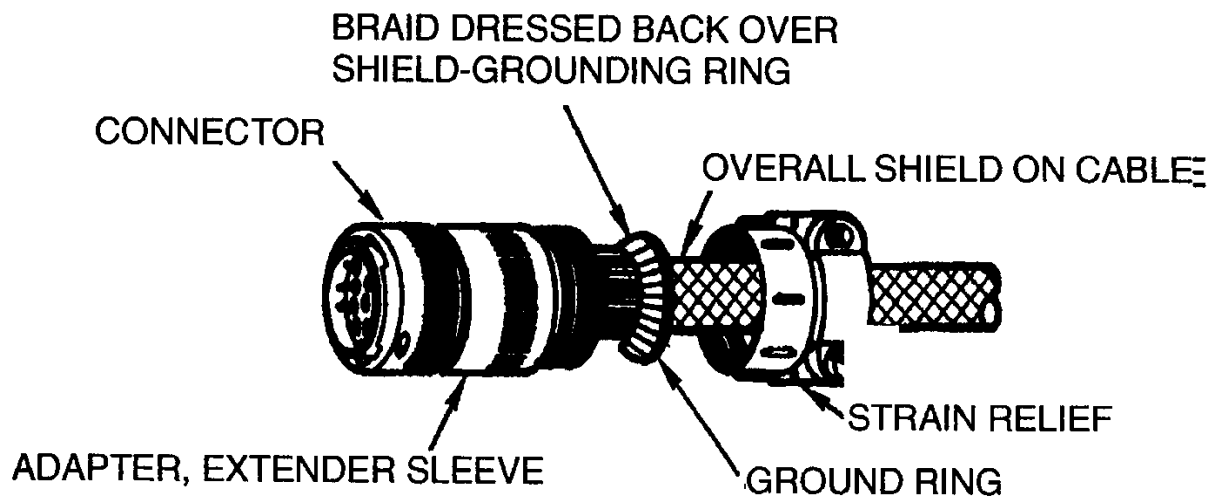
Figure Error! No text of specified style in document.-18. Terminating Overall Shield in RFI Adapter (Typical)
