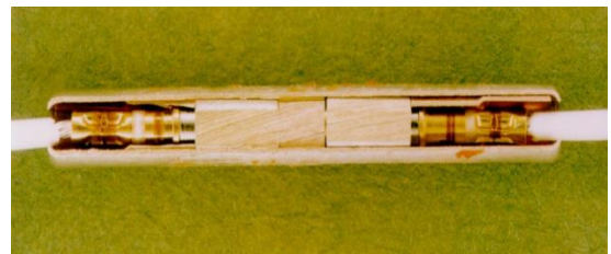
Figure Error! No text of specified style in document. -62. Crimped Contacts Inserted Into Junction Device
