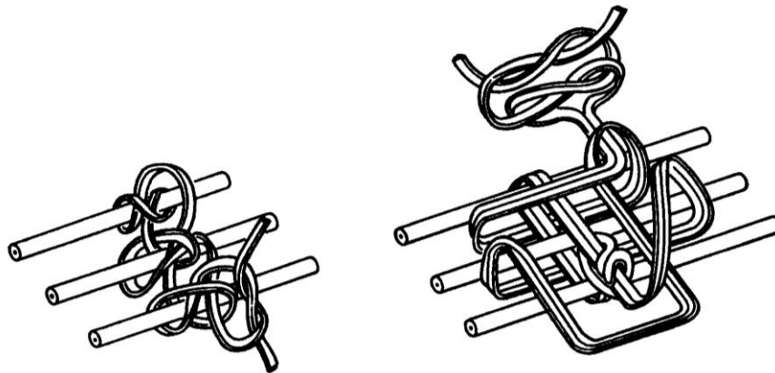
Figure Error! No text of specified style in document. -8. Flat Lacing Stitches
