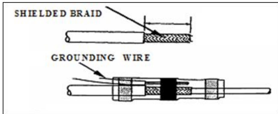
Figure Error! No text of specified style in document.-32. Individual Shield Termination with a Lap Splice and Solder Sleeve
