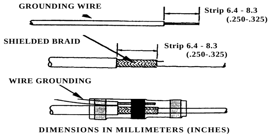
Figure Error! No text of specified style in document.-19. Example of Individual Shield Termination Using a Heat Shrinkable Solder Sleeve
