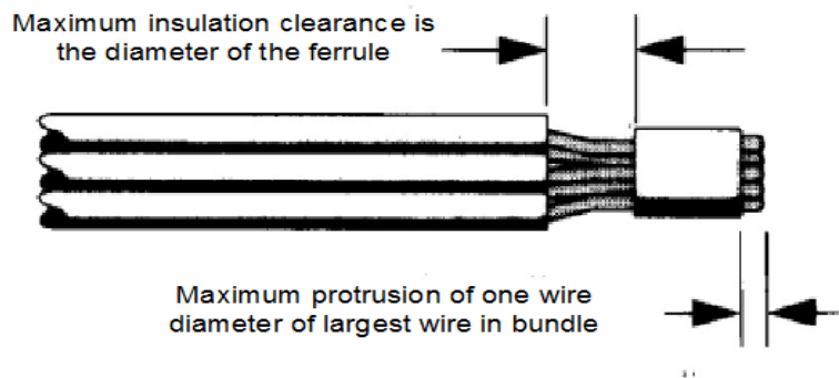
Figure Error! No text of specified style in document.-48. Solder Ferrule
