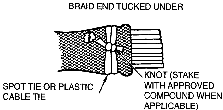
Figure Error! No text of specified style in document. -9. Securing Fabric Braid Sleeving
