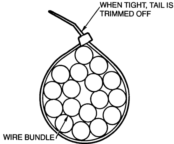
Figure Error! No text of specified style in document.-14. Plastic Strap Orientation
