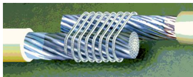
Figure Error! No text of specified style in document.-36. Lashing of Pre-Tinned Conductors
