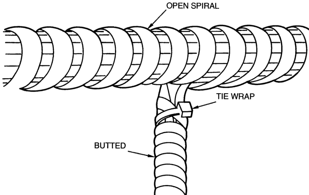
Figure Error! No text of specified style in document.-13. Spiral Wrap Sleeveing
