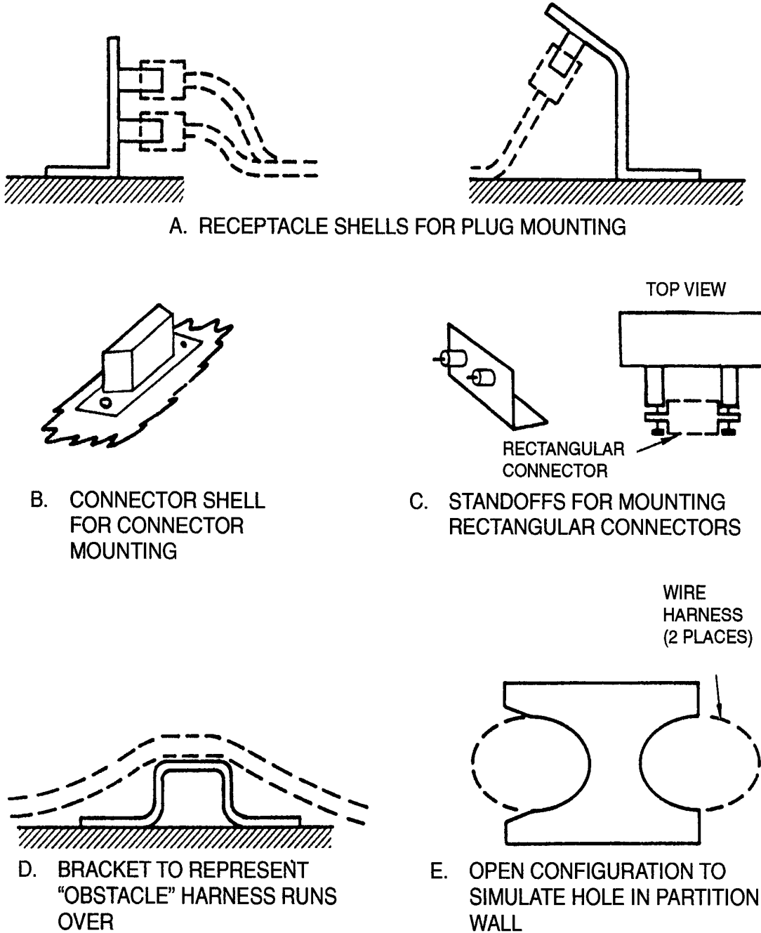
Figure Error! No text of specified style in document.-2. Typical Harness Board Hardware and Fixtures
