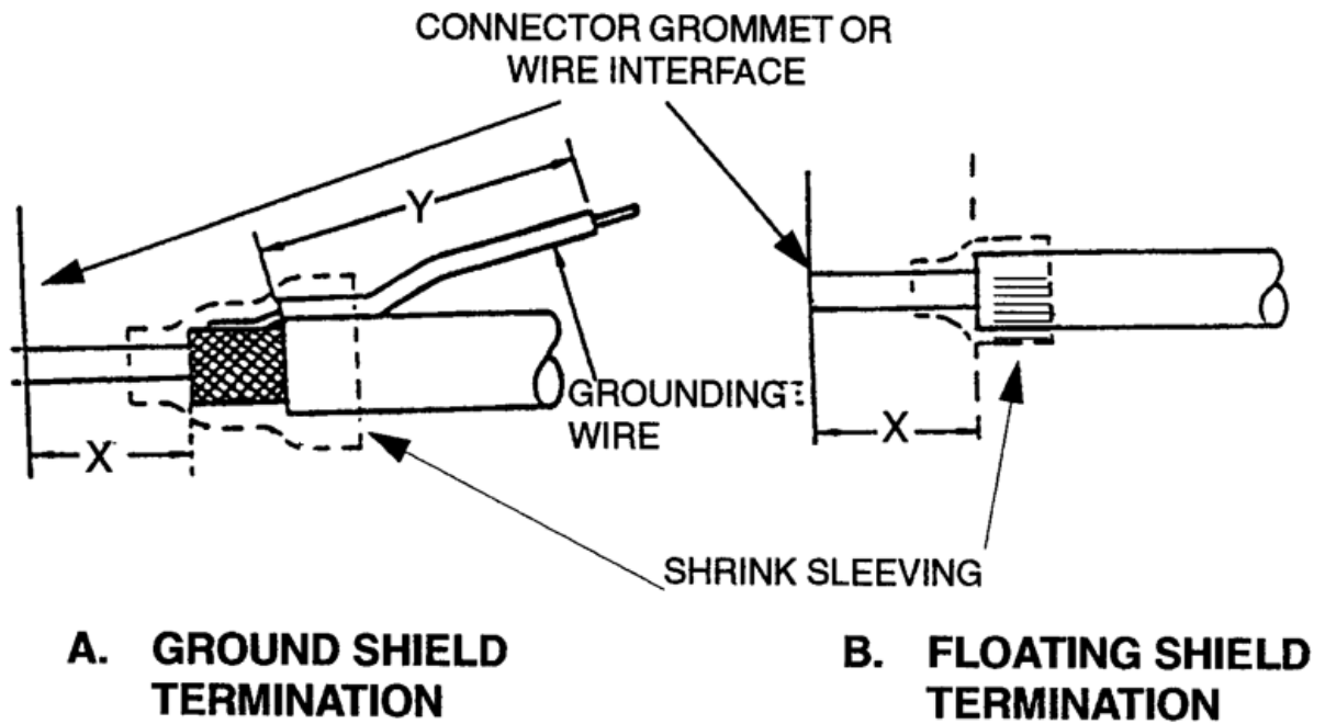
Figure Error! No text of specified style in document.-25. Conductor Exposure for Individual Shield Termination Types
