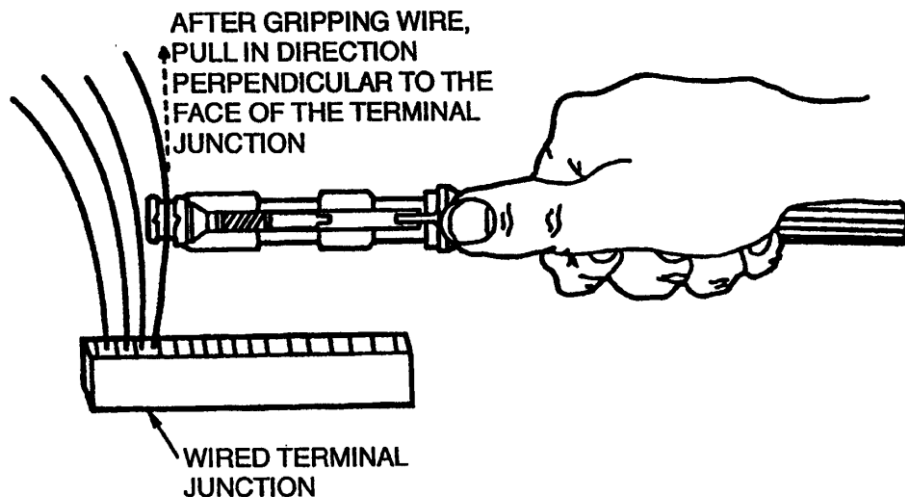
Figure Error! No text of specified style in document.-28. Application of Retention Tool for Gripping Wire (Typical)
