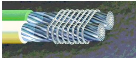
Figure Error! No text of specified style in document.-39. Lash End Type Splice
